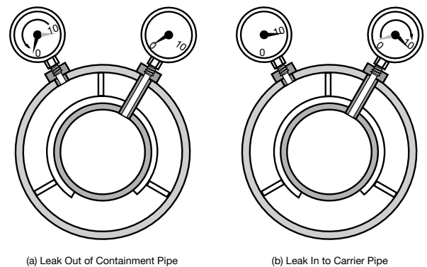
Figure F-98. Annular pressure test leak indications
