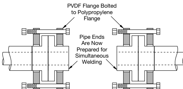
F Figure F-109. Bolt polypropylene flanges to PVDF flanges
