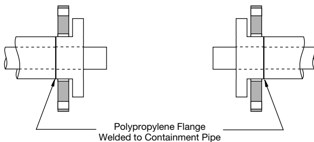
F Figure F-108. Weld polypropylene flanges to pipe ends
