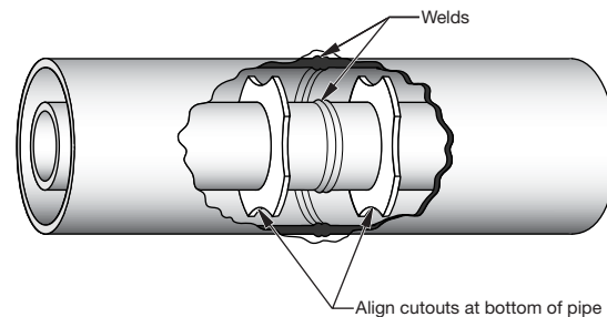
Figure F-93. Support disc alignment
