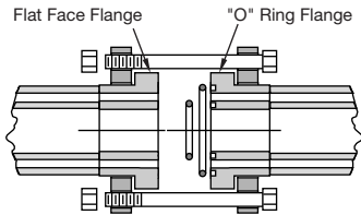
Figure F-100. Double-wall flange
