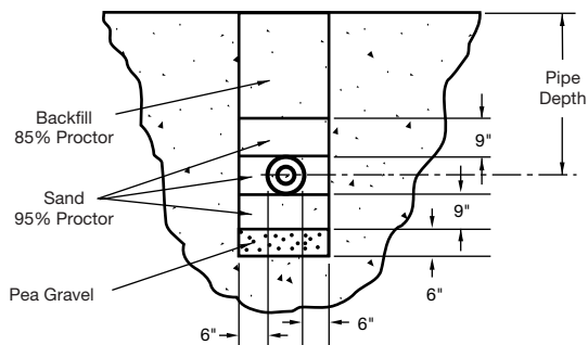
Figure F-97. Trench detail
