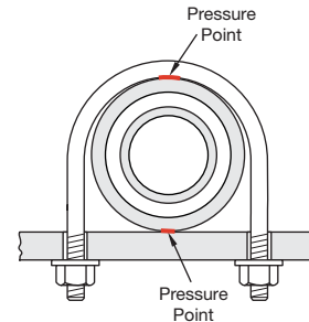
Figure F-95. Effects of U-bolt on pipe—not recommended
