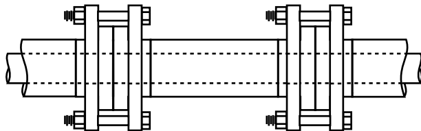
Figure F-103. Install flanged spool
