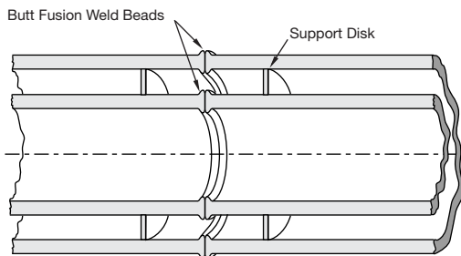
Figure F-94. Typical butt-fusion weld bead
