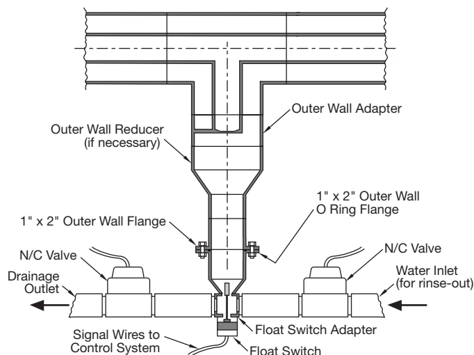
Figure D-25. Drain and low point Poly-Flo system
