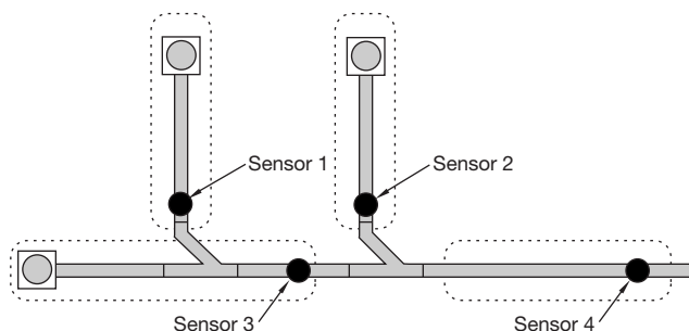
Figure D-29. Sample locations for low point sensors
