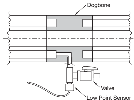
Figure D-26. Simple connection, Duo-Pro/Fluid-Lok systems
