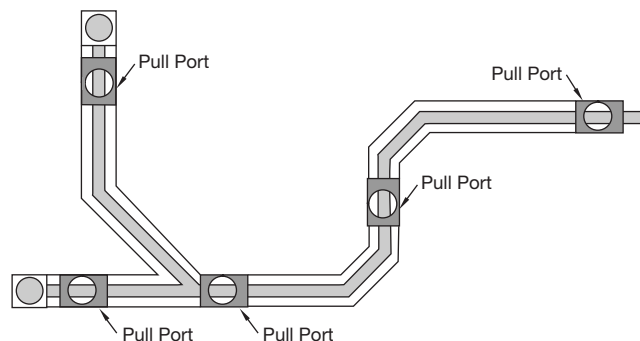
Figure D-34. Pull port locations for leak detection cable
