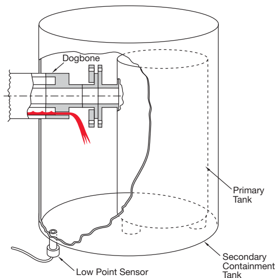
Figure D-28. End-of-line connection option, Duo-Pro/Fluid-Lok systems
