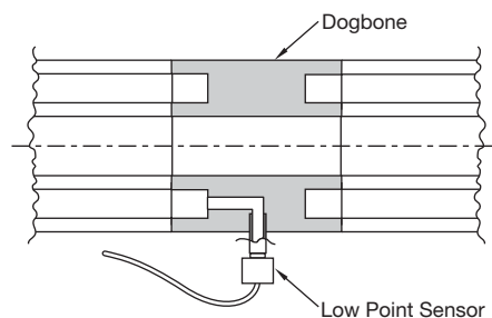
Figure D-26. Simple connection, Duo-Pro/Fluid-Lok systems
