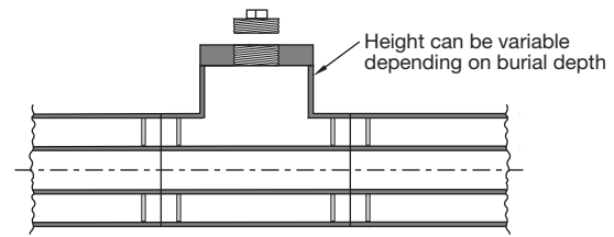
Figure D-32. Access tee with threaded cover
