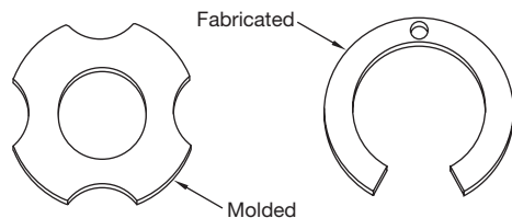
Figure D-31. Two typical end of pipe support discs to accommodate leak detection
