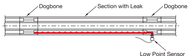
Figure D-30. Leak detection compartments
