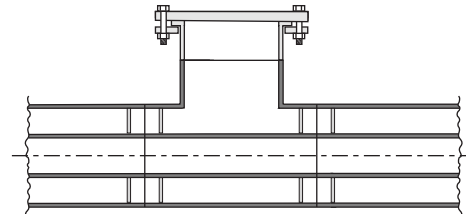
Figure D-33. Access tee with flanged cover
