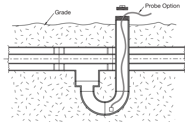
Figure D-37. In-line inspection well
