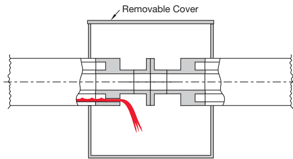
Figure D-38. End-of-line inspection well
