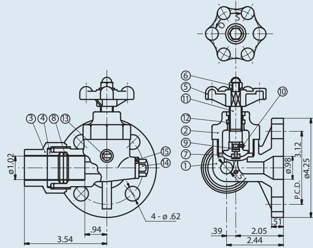
1" GAUGE VALVE
