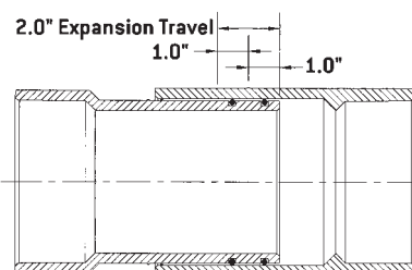
Expansion Joint - Charlotte Part No. 133
